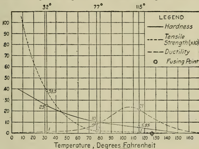
FIG. 111.—Chart of Physical Characteristics of Blown Petroleum Asphalt.
